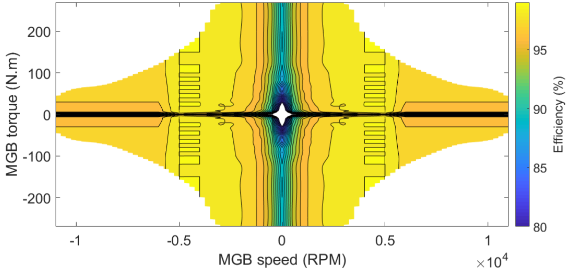
Figure 22. TPIM Inverter B Efficiency
