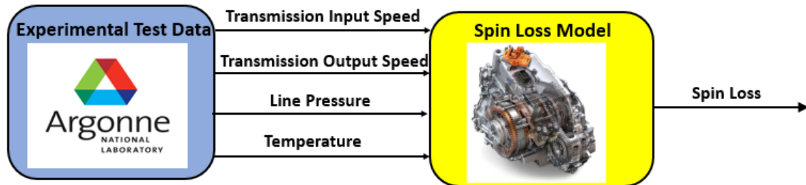
Figure 33. Transmission Spin Loss model
