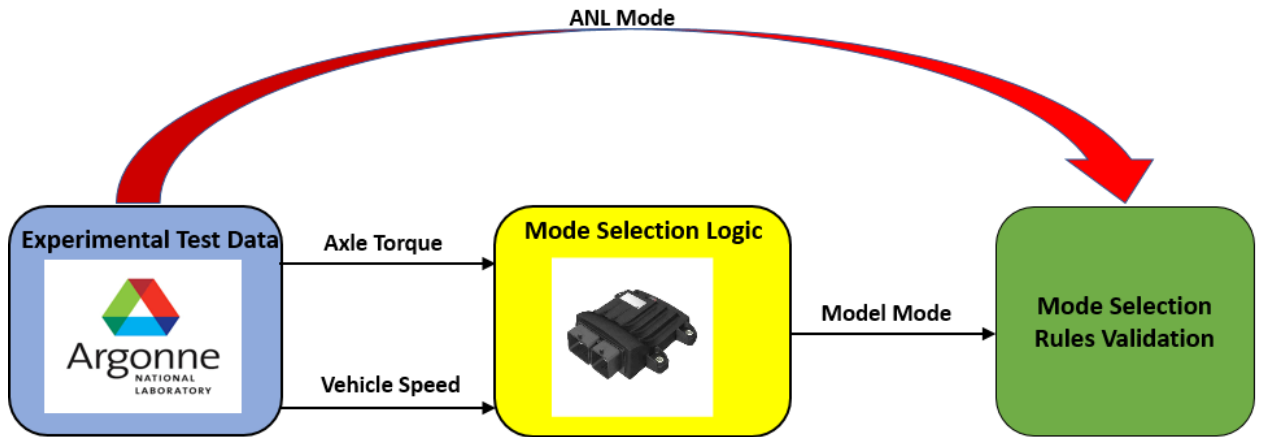
Figure 38. ANL Mode Selection Logic Validation
